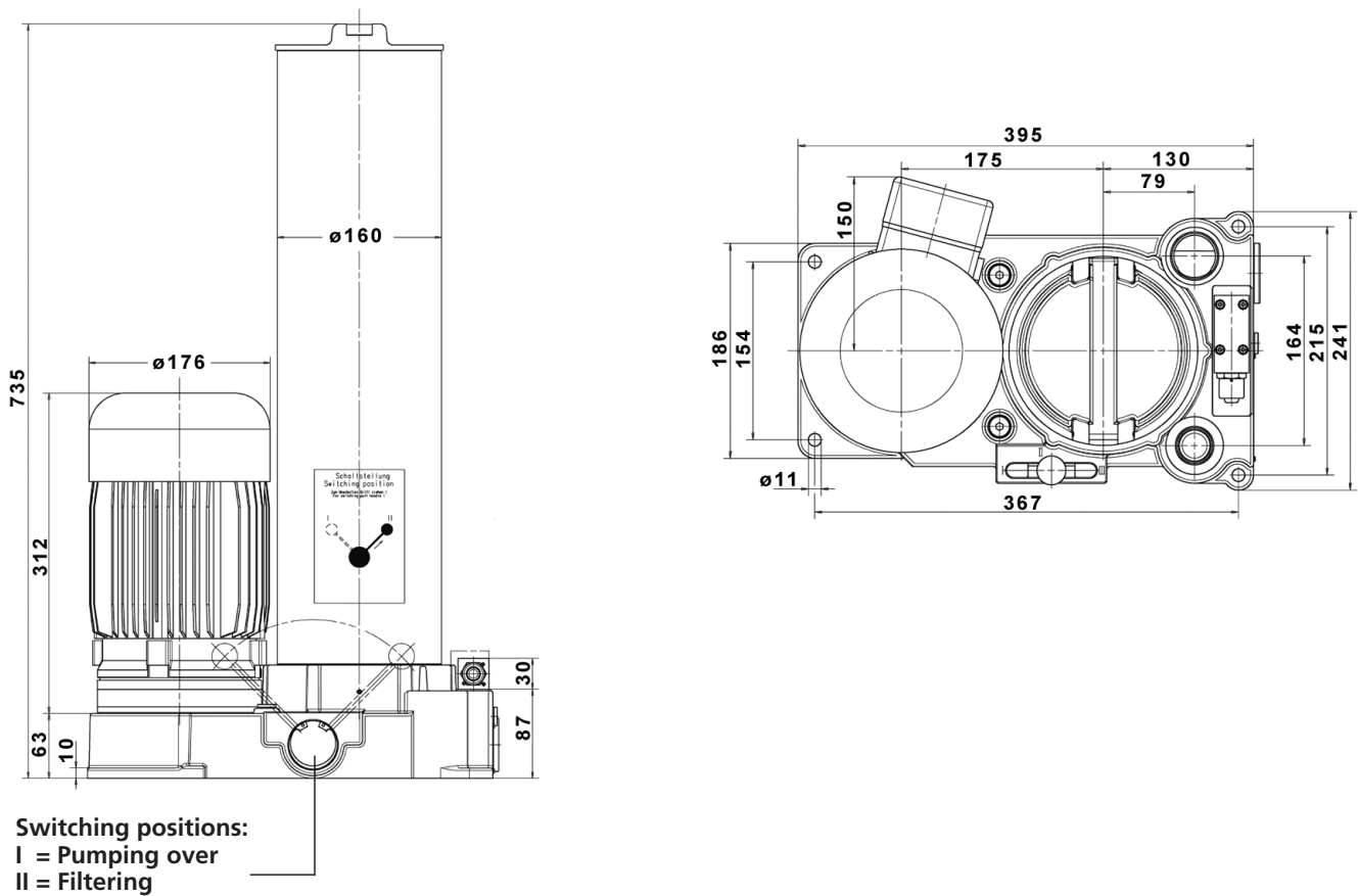
Fig. 11: Device dimensions
